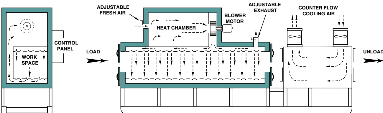
Full vertical air flow forces heated air down through parts.
