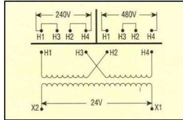
CONNECTION DIAGRAM: GROUP "B"
