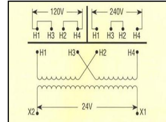
CONNECTION DIAGRAM: GROUP "C"
