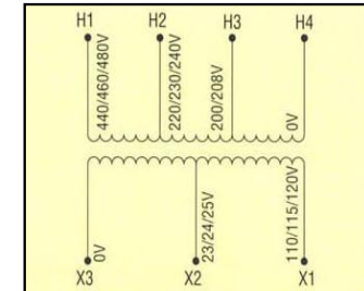
CONNECTION DIAGRAM: GROUP "F"
